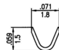
B-B SECTION
